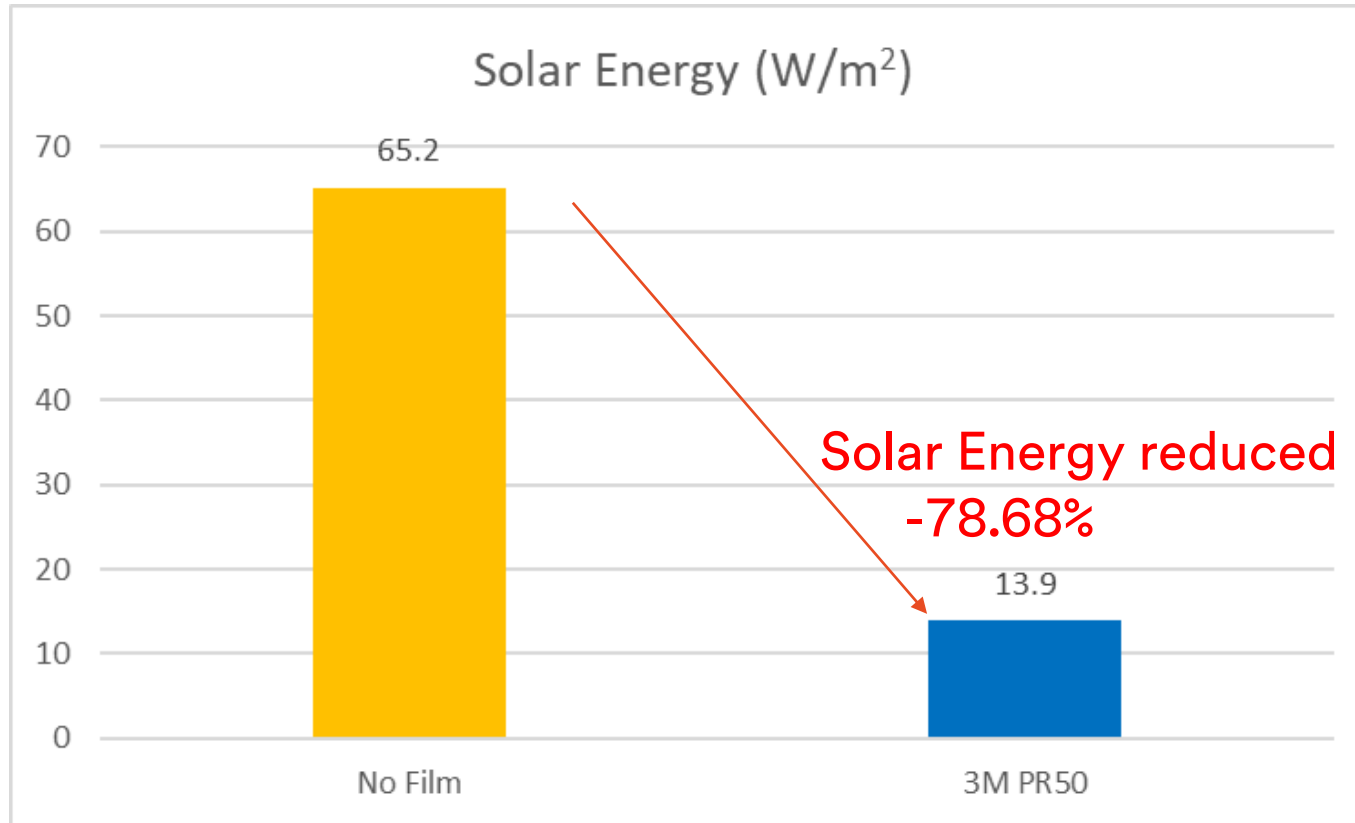
Solar Energy measured by Solar Power meter
