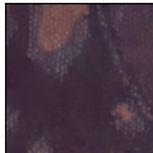
Ours 29.81/0.659
