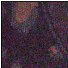
Noisy 17.68/0.172
