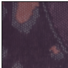
MPRNet 31.06/0.733
