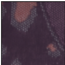
MIRNet 31.21/0.733
