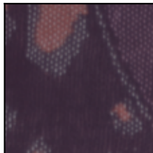
Uformer 31.27/0.738
