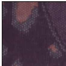
NAFNet 31.97/0.775
