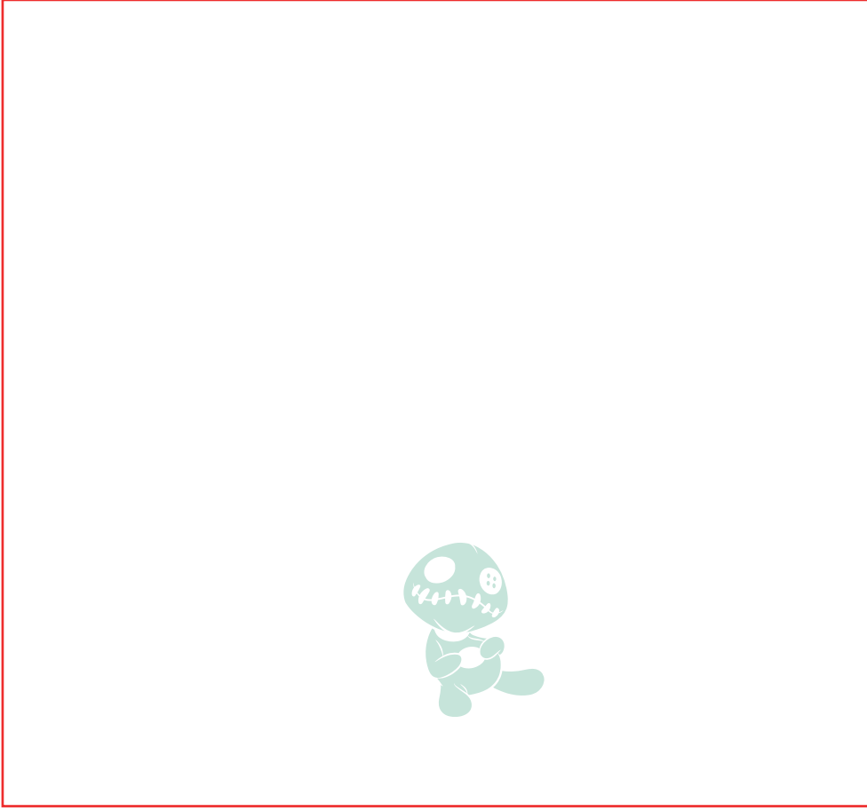
PANTONE 12-5407 TPX
