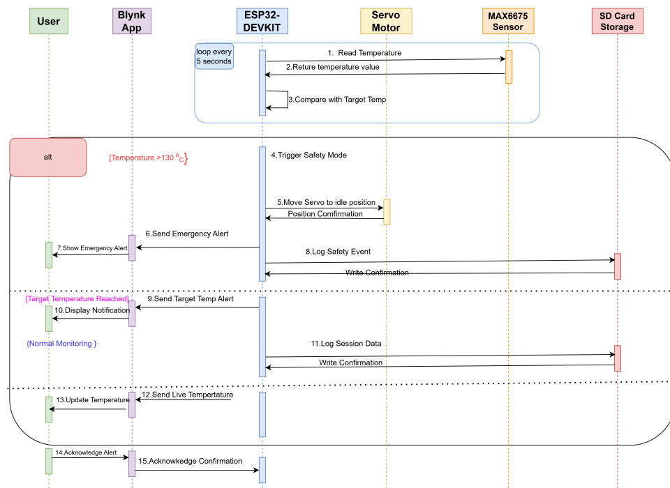
Figure 12: Sequence Diagram: Temperature Alert
