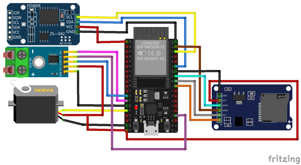
Figure 4: SolarTrace Wiring Diagram (Fritzing)
