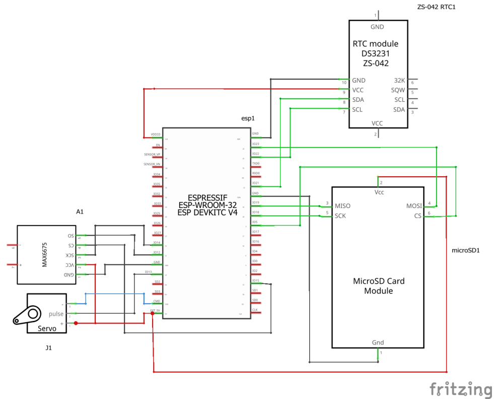
Figure 3: Complete System Schematic Diagram
