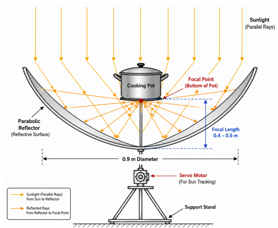
Figure 5: Parabolic Dish Geometry and Sunlight Concentration
