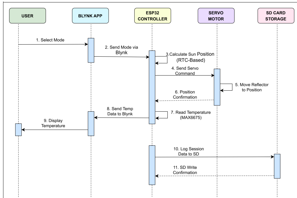
Figure 11: Sequence Diagram: Mode Selection
