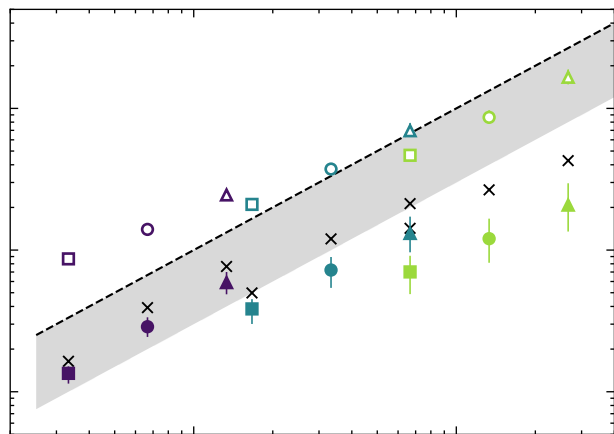
3 \times 10^{11} M_{\odot} : AGN + stellar wind on
