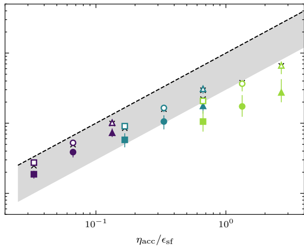
3 \times 10^{11} M_{\odot} : AGN + stellar wind on
