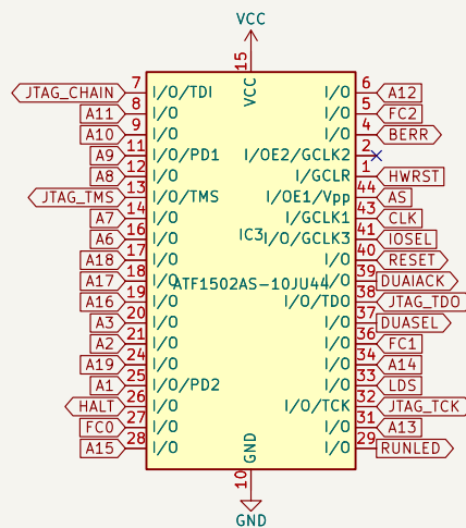
IC3: code/pld/cpld/ic3_glue.pld
