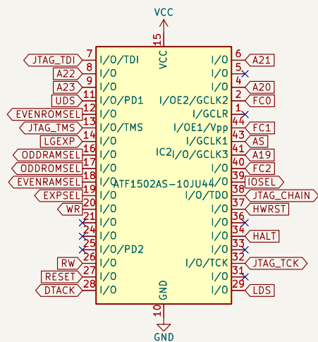
IC2: code/pld/cpld/ic2_decoder.pld
