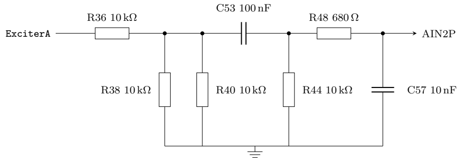
Figure 3: Input network of channel A, as built on REV B ( R_{48} is 680 \Omega , not the 680 \text{ k}\Omega of the schematic). Channel B is identical ( R_{37} , R_{39} , R_{41} , C_{54} , R_{45} , R_{49} , C_{58} ) and ends at \text{AIN1P} . The ADC's negative inputs are tied to ground.
