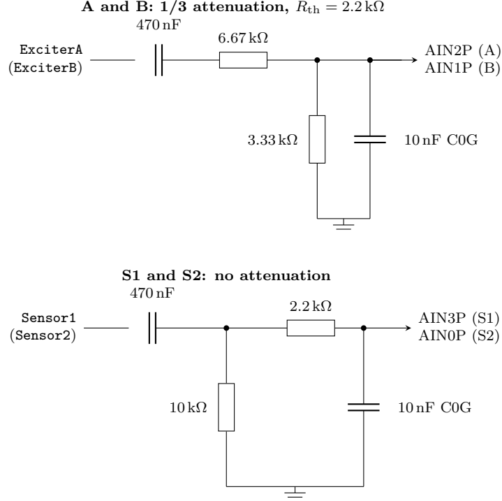
Figure 7: Planned REV C input networks. The 6.67 k/3.33 k pair is one matched resistor network (10 k total, ratio 2:1). All coupling capacitors are 470 nF, all pin capacitors 10 nF C0G.
