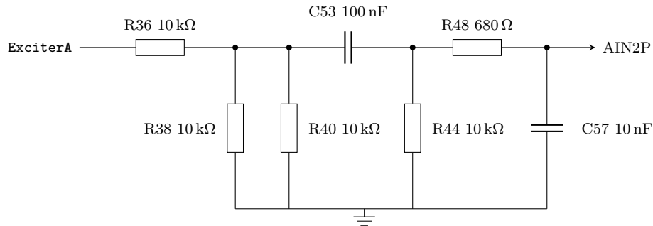
Figure 3: Input network of channel A, as built on REV B (R48 is 680 \Omega , not the 680 \text{ k}\Omega of the schematic). Channel B is identical (R37, R39, R41, C54, R45, R49, C58) and ends at AIN1P. The ADC's negative inputs are tied to ground.
