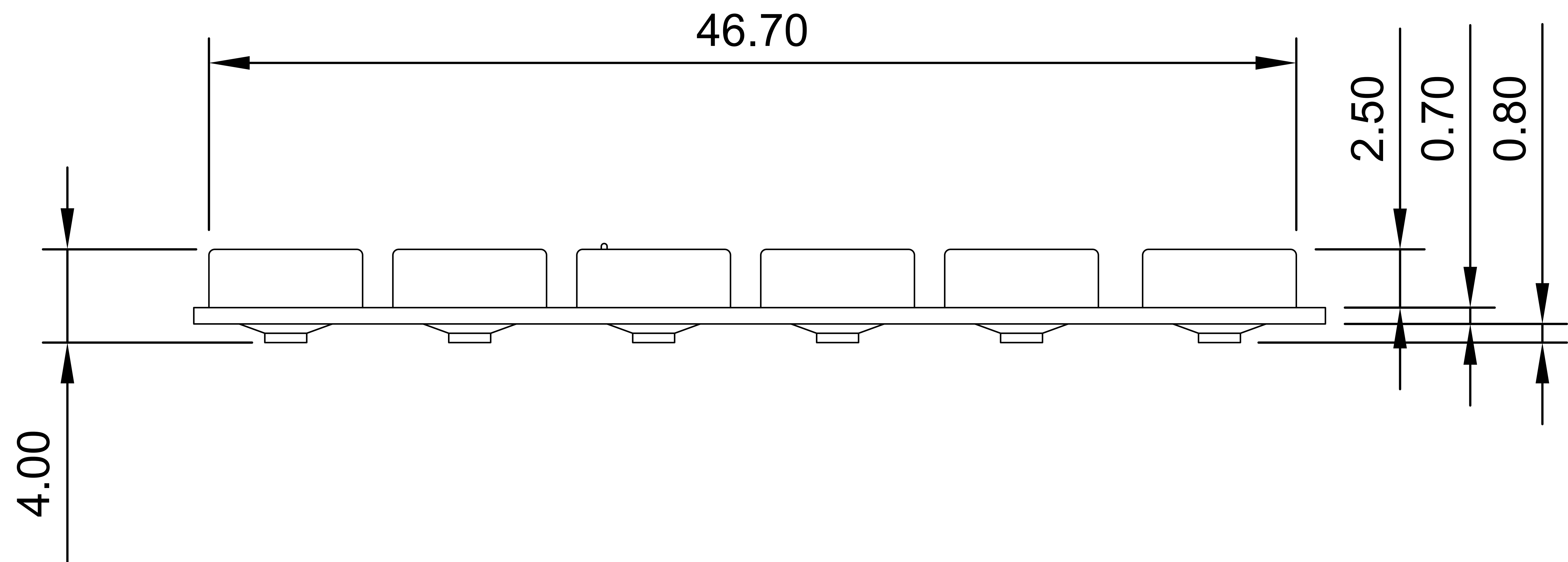
Keypad Side View unit: mm
