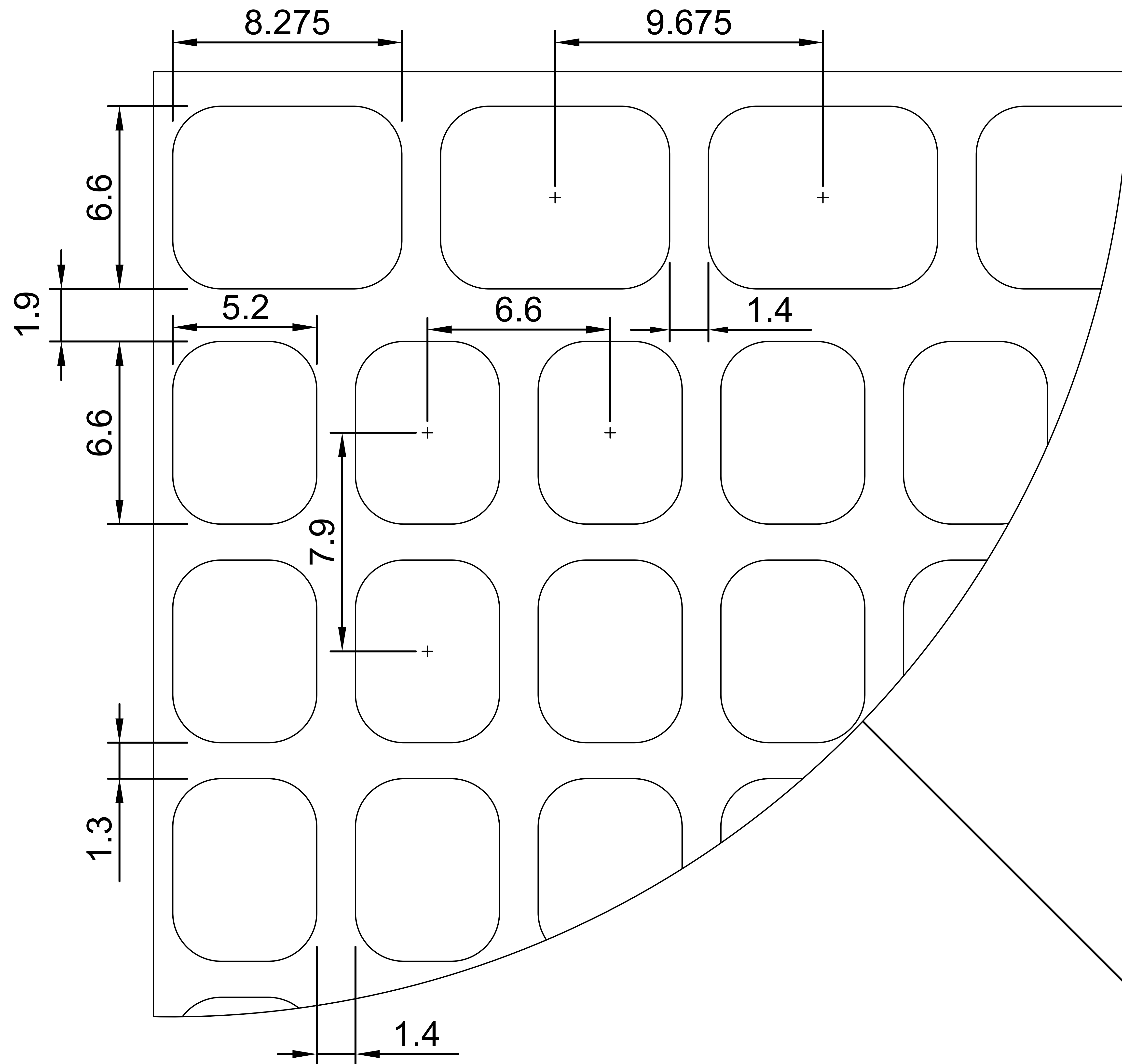
Keypad Front View Fragment unit: mm
