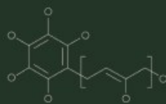
coenzyme q 10
