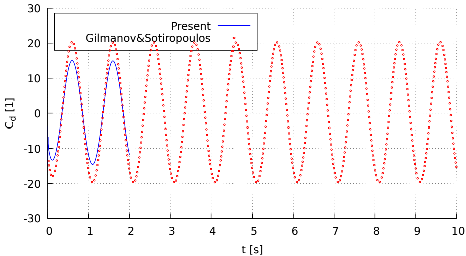
Drag Coefficient ( C_d ) vs. Time ( t )
