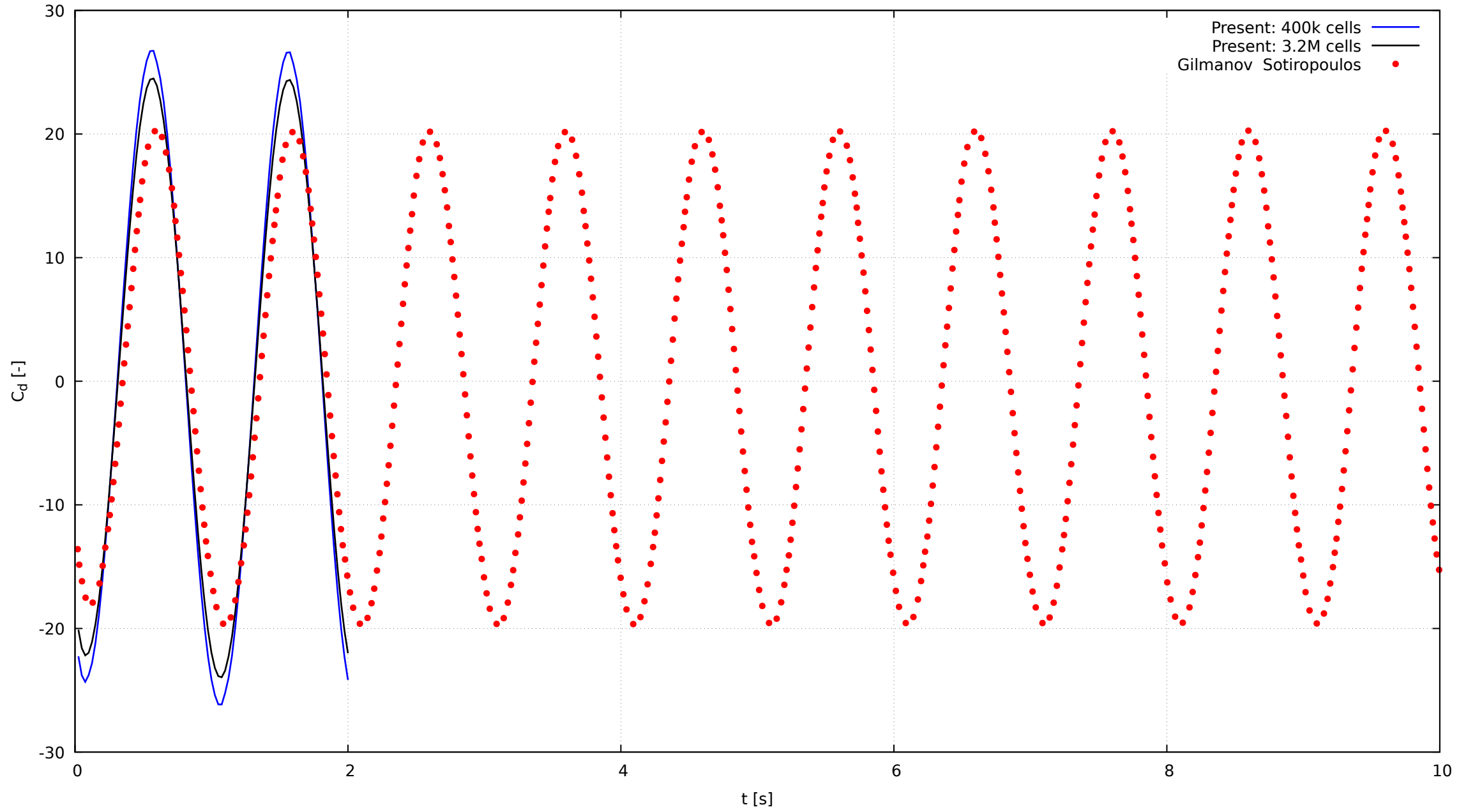
Oscillating sphere: drag coefficient comparison
