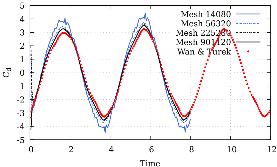
Oscillating Cylinder Drag Coefficient Comparison
