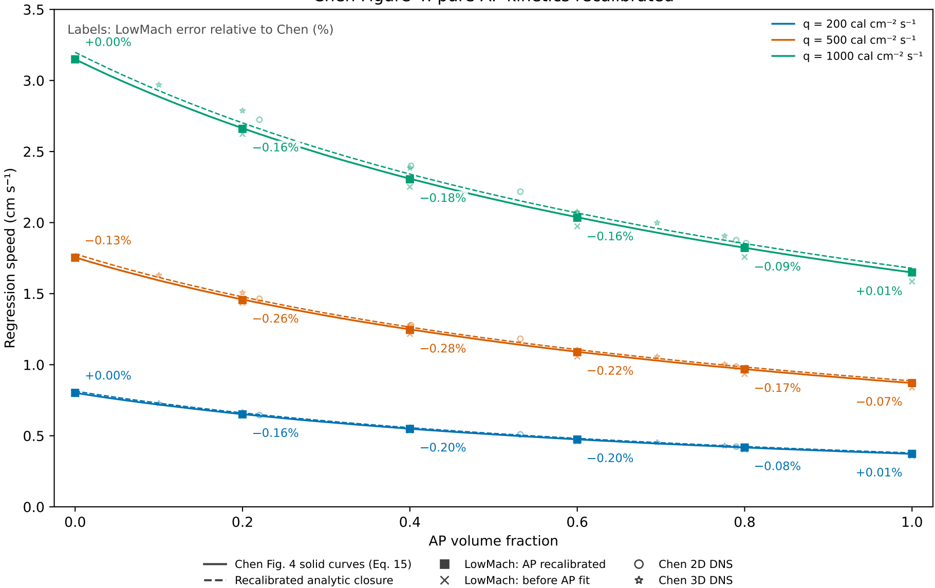
Chen Figure 4: pure-AP kinetics recalibrated
