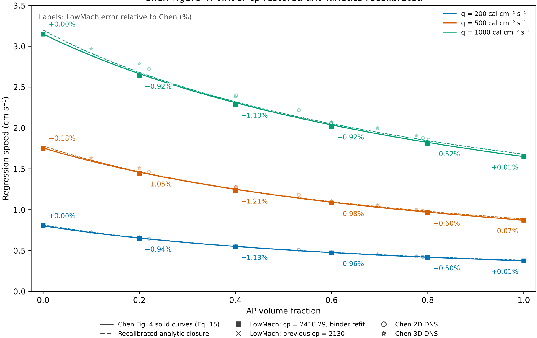
Chen Figure 4: binder cp restored and kinetics recalibrated
