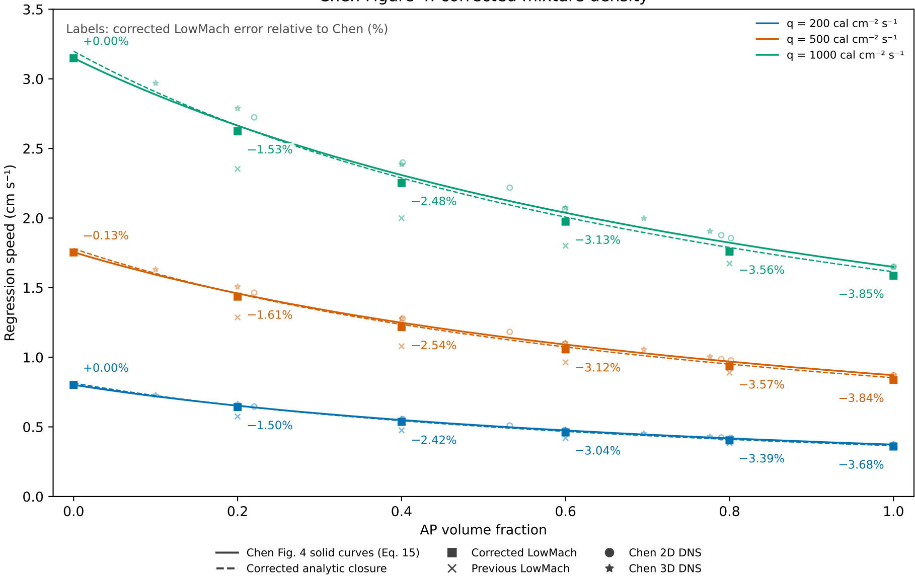
Chen Figure 4: corrected mixture density
