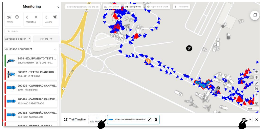
Figure 4 – Trace – Timeline
