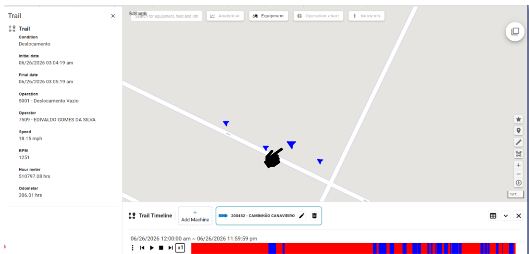
Figure 5 – Pop-up Trail
