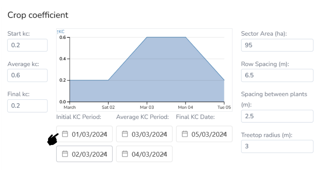
Figure 5 – Standardized dates for DD/MM/YYYY in the Crop Coefficient (KC) – Configurations tab.
