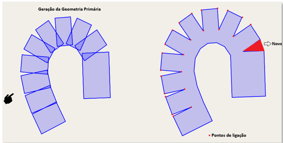
Figure 11 – Before and after model of the improvement in the geometry of the sharp curves
