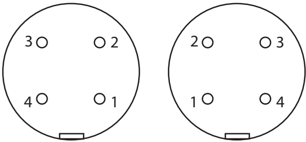
Female HR10A-7P-4S(73) Male HR10A-7P-4P(73)
