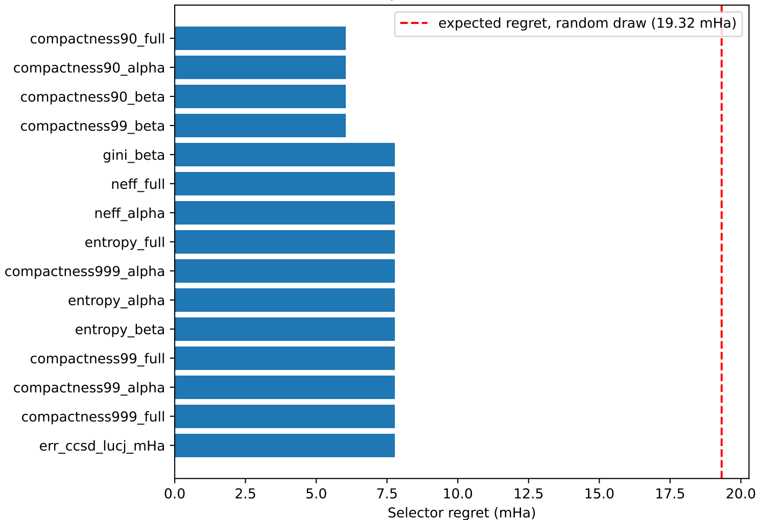
Predictor selection regret vs subspace error (15 best predictors; lower is better)
