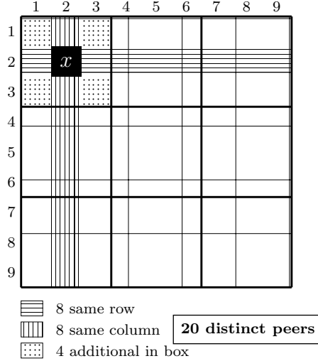
Figure 3: The 20 distinct peers of cell x : eight cells in the same row, eight in the same column, and four additional cells in the same 3 \times 3 box.
