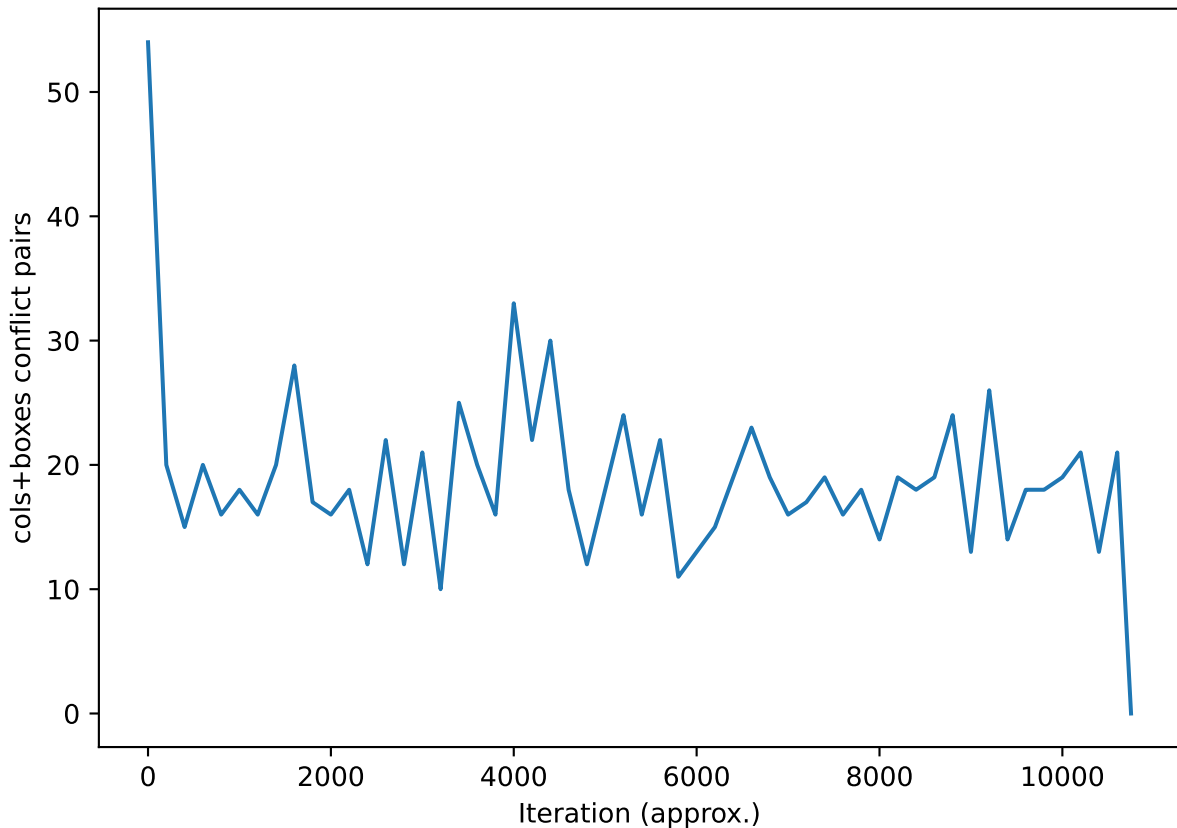
Loss trajectory (clues=30, seed=115642242)
