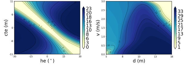
Figure 3: Visualization of the synthesized SBCs in verification-Guided training for X-Plane11 Trajectory Tracking (left) and CARLA Emergency Braking (right).
