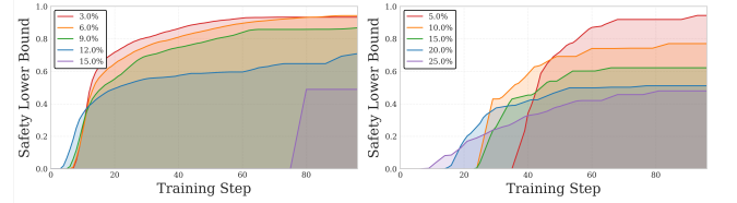
Figure 4: Maximum verifiable safety probability vs. training steps under different disturbances for X-Plane11 Trajectory Tracking (left) and CARLA Emergency Braking (right).
