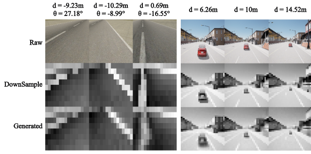
Figure 2: Comparison of Perception model approximations in the X-Plane11 (left) and CARLA (right) simulation environments. Each group displays the raw input, downsampled image, and generated grayscale image. The corresponding state parameters, distance d (m) and heading angle \theta ( ^\circ ), are shown above.
