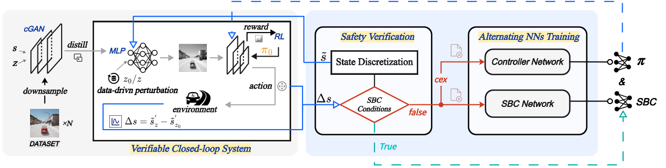
Figure 1: The pipeline of SafePVC. The left block presents the observation approximator , which uses a cGAN-based state–image mapping and RL-based pretraining to construct a verifiable closed-loop system (VCLS) with an initial controller \pi_0 . After obtaining \pi_0 , the VCLS executes under environmental perturbations to obtain a data-driven state disturbance distribution. This distribution, together with the full VCLS, is then passed to the controller generator in the right block. The pretrained controller is evaluated by synthesizing an SBC that certifies probabilistic safety under disturbance \Delta s derived from discretized states \tilde{s} . If the SBC violates posterior feasibility, counterexamples (cex) are extracted to alternately refine both the controller and SBC networks. The refined controller is reinserted into the VCLS to update the disturbance distribution, and this loop continues until both a valid SBC and a controller \pi with provable probabilistic safety are obtained.
