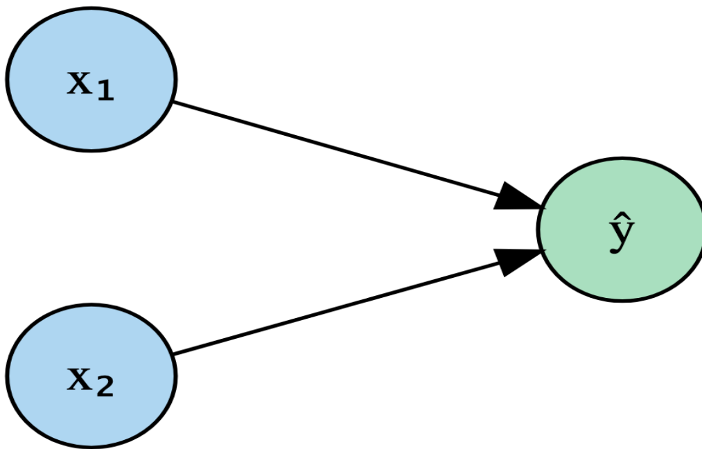
Figure 8.1: A network with no hidden layers is equivalent to linear regression: the output is a linear combination of the inputs.
