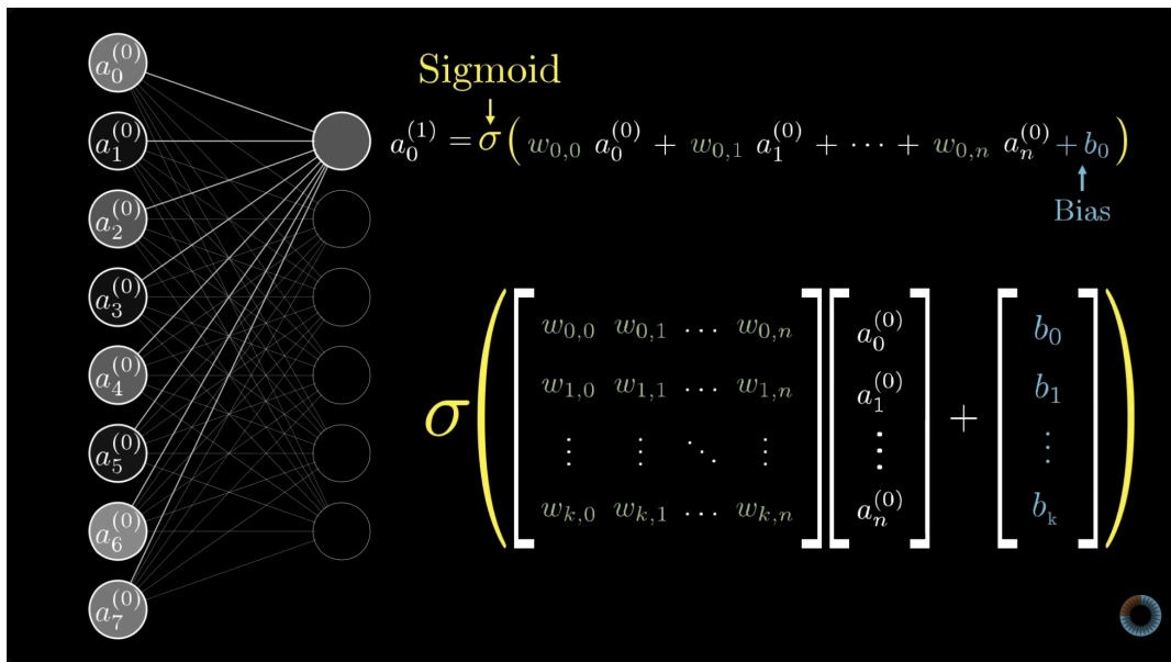
Figure 8.4: One layer of the forward pass written out in full: the weighted sum for a single neuron (top) and for every neuron in the next layer at once (bottom). Source:
