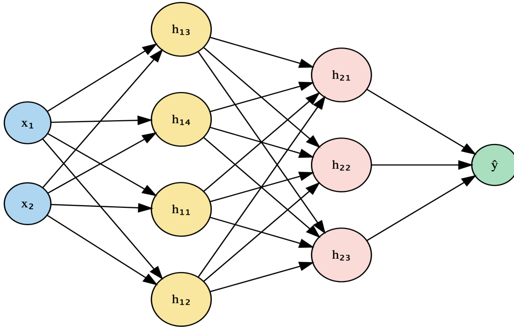
Figure 8.3: A network with two hidden layers. Each layer refines the representation of the previous layer, enabling hierarchical feature construction.
