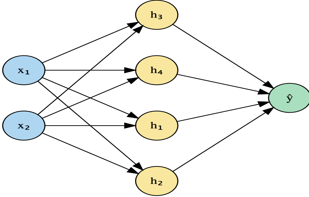
Figure 7.2: A network with one hidden layer. Each hidden neuron applies a nonlinear activation function to a weighted sum of the inputs.
