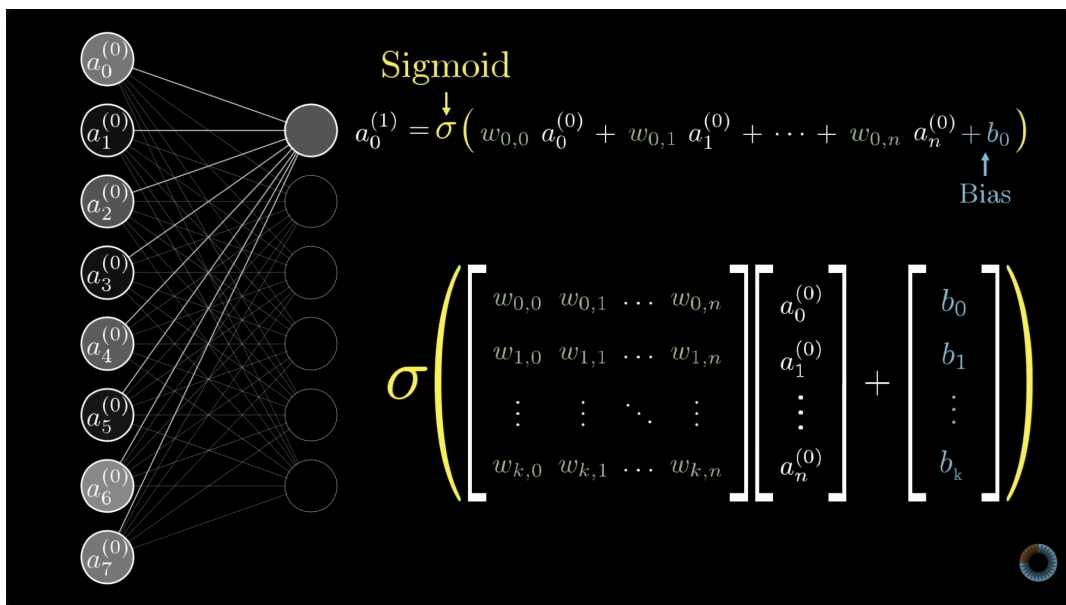
Figure 7.4: One layer of the forward pass written out in full: the weighted sum for a single neuron (top) and for every neuron in the next layer at once (bottom). Source:
