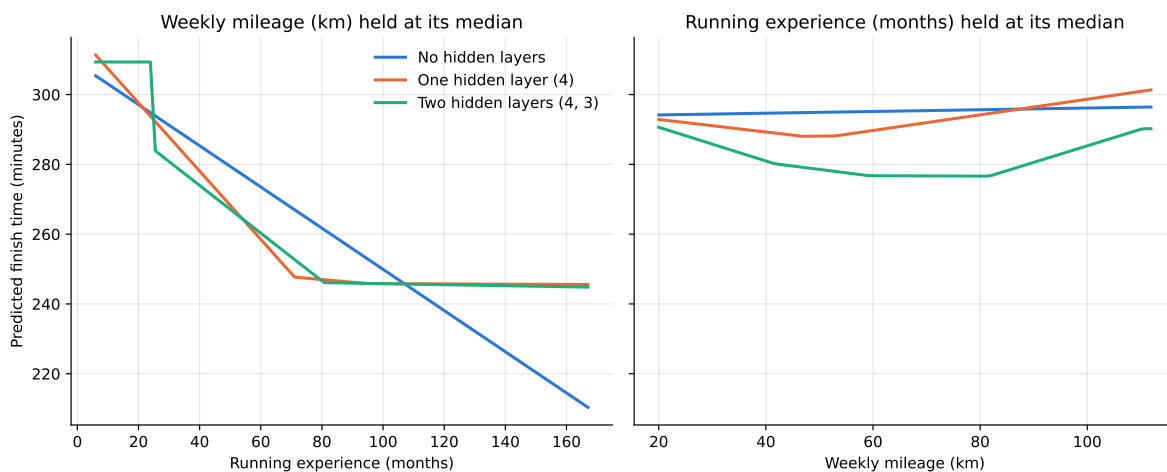
Figure 7.6: Partial effects of each predictor for the three networks. Left: running experience varies with weekly mileage held at its median. Right: weekly mileage varies with running experience held at its median.
