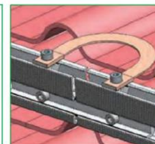
Item No.: ING-BJP Material: Copper Size: 20mm X 150/250mm Site: Aluminum rail or C-channel
