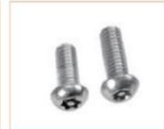
Name: Anti-Theft Bolt Material: SUS304 Size: M 8x 20-60
