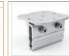
Longline 305 Clamp Item No.: ING-MRB-L305 Material: AL6005-T5 Roof: Longline 305 roof
