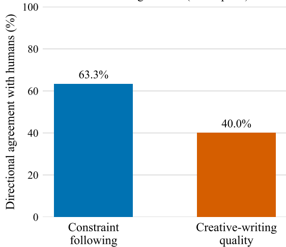
A. Human-LLM agreement (N=30 pairs)
