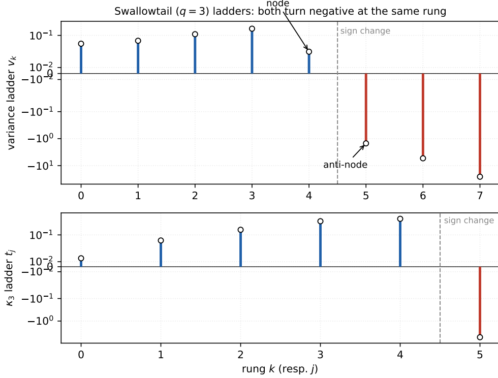
FIGURE 1. The two swallowtail ladders (symlog scale, blue +, red -). Top : the variance ladder (3), with the near-node at |v_4| \approx 0.036 and the anti-node at |v_5| \approx 1.50 marked. Bottom : the \kappa_3 ladder (5) on its own scale. Both first turn negative at the same rung k = 5 (dashed line) — the shared \cos(k\theta - \varphi) envelope of Claim 11, two rungs later than the cusp's. Note the node ( k = 4 ) and the sign change ( k = 5 ) are distinct for the swallowtail, unlike the cusp where both fall at k = 3 .
