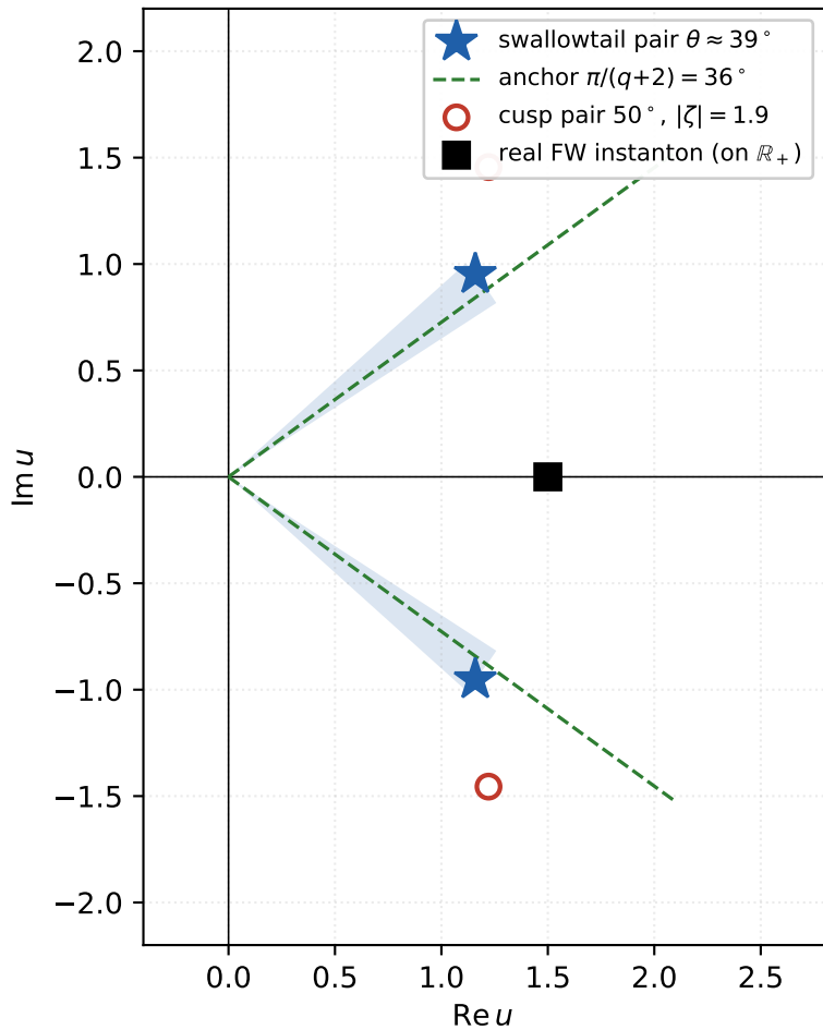
Borel plane of the swallowtail law
