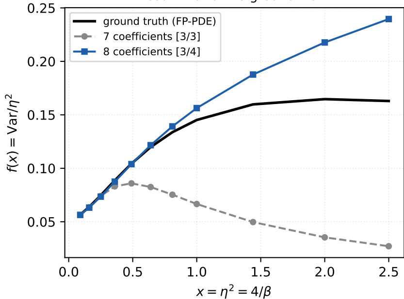
Resummation vs ground truth
