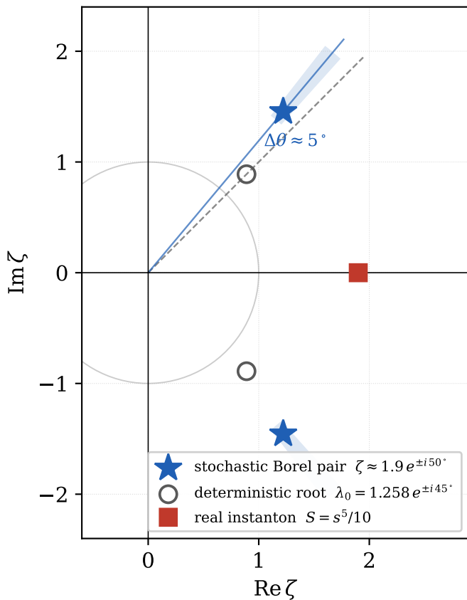
Borel plane of \mathcal{W} : conjugate pair + real instanton
