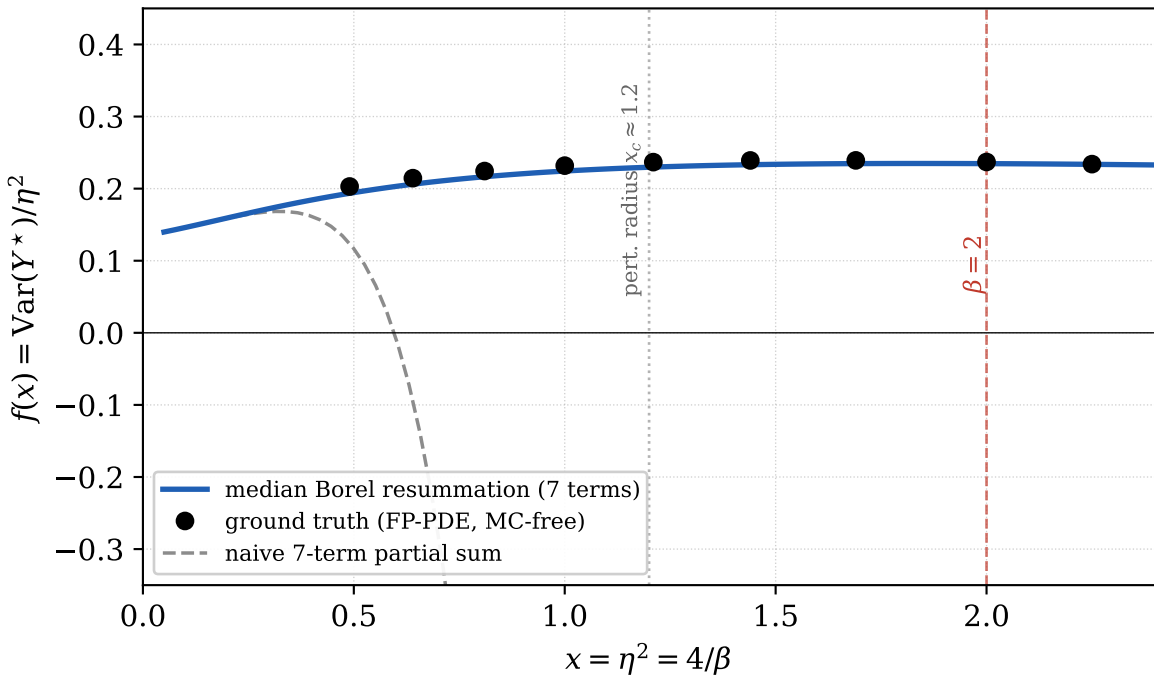
Resummed trans-series reconstructs \mathcal{W} beyond the radius
