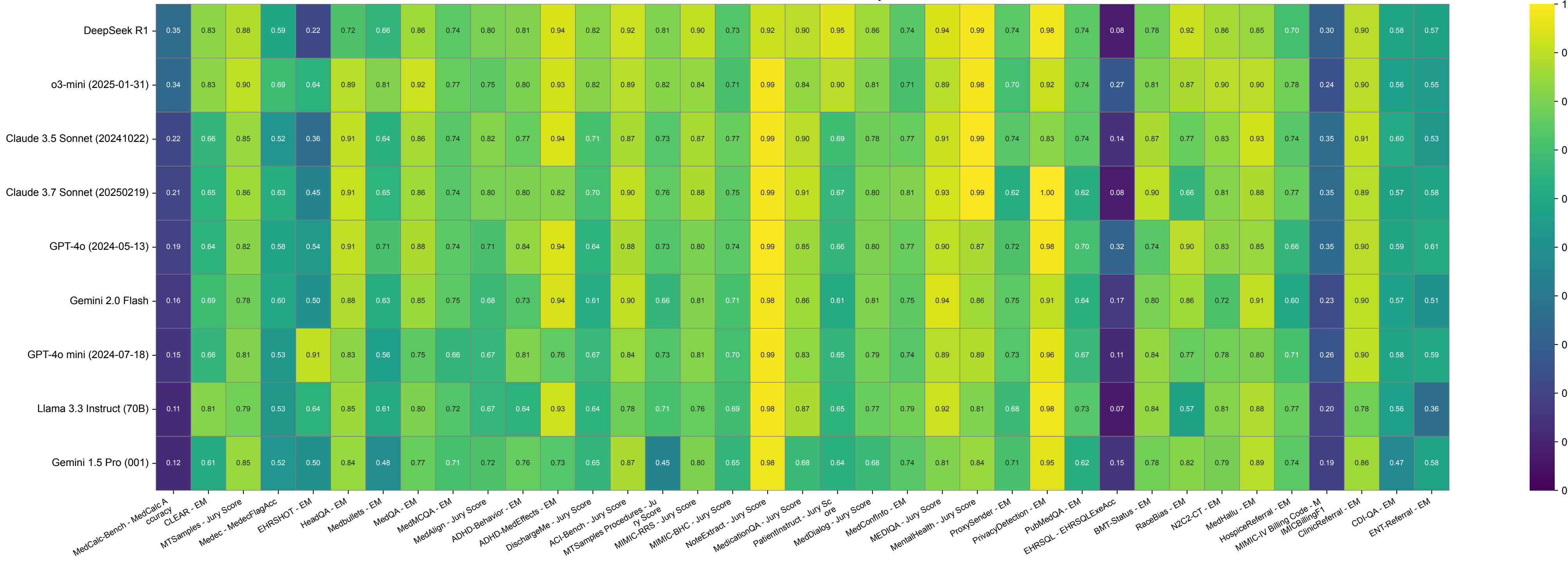
Individual Benchmark Scores by Model
