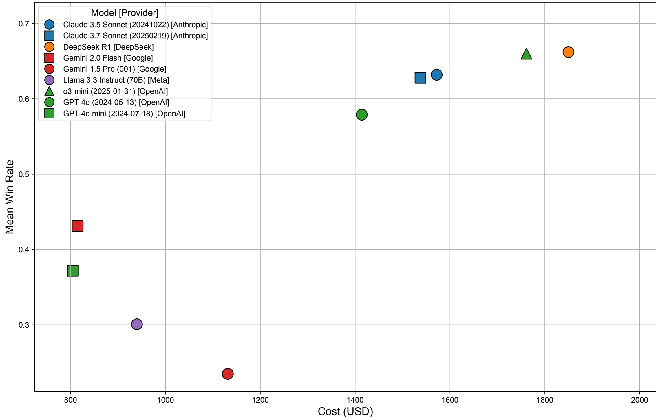
Cost vs Mean Win Rate
