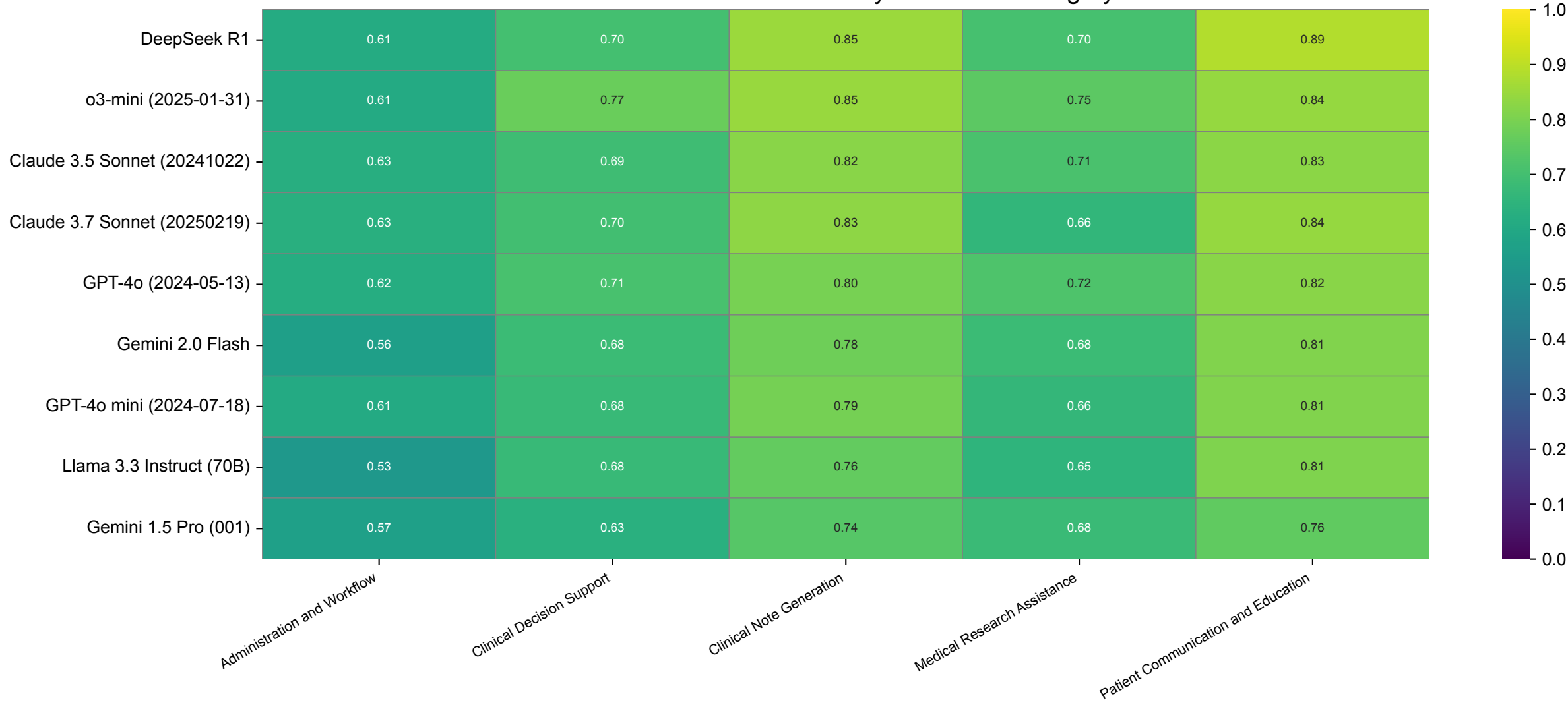
Mean Normalized Scores by Model and Category
