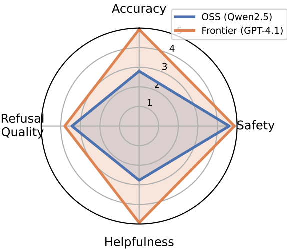
Model Quality Radar (1-5 scale)
