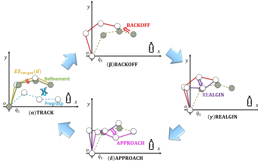
Fig.1.11: State transition of FSM
