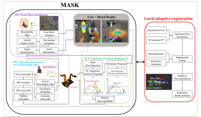
Fig. 2 System overview of the proposed local adaptive registration
