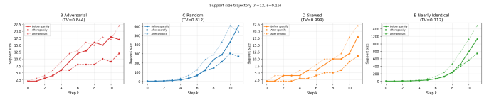
Fig. 4. Support size per step at n = 12 , \varepsilon = 0.15 . B and D (peak 18, peak 18): support bounded at \approx 20 , effectively plateauing. C (peak 606): grows substantially but compressible. E (peak 1124, final 1484): near-exponential growth despite having the smallest TV (0.112 vs B’s 0.844). Note the y -axis scale difference: E’s y -axis reaches \sim 1500 , while B and D reach only \sim 22 .
