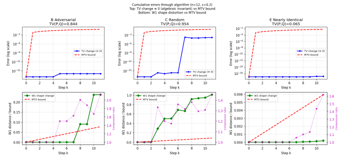
Fig. 3. Cumulative errors through the deterministic algorithm ( n = 12 , \varepsilon = 0.2 ). Top row: TV change (blue, \equiv 0 at machine precision \leq 10^{-15} ) vs MTV bound (red dashed, rising linearly). Bottom row: W_1 shape distortion (green) vs MTV bound. B: final W_1 = 0.237 , bound= 0.077 (tightness 3.07). C: final W_1 = 1.008 , bound= 0.087 (tightness 11.5). E: final W_1 = 1.8 \times 10^{-4} , bound= 0.006 (tightness 0.03).
