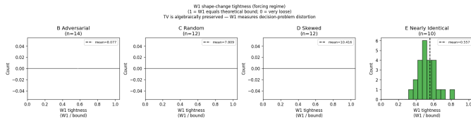
Fig. 1. W_1 tightness ( W_1/\text{bound} ) at the forcing regime ( \varepsilon_s = 0.3 , n = 14 for B, n = 12 for C/D, n = 10 for E). Families B, C, D show W_1 \gg \text{bound} (means 8.1, 7.8, 10.4; histograms all fall at 0 on the [0,1] scale because W_1/\text{bound} > 1 ). Family E is the only family where W_1 < \text{bound} (mean=0.557), showing the MTV bound is genuinely conservative for near-1 merging.
