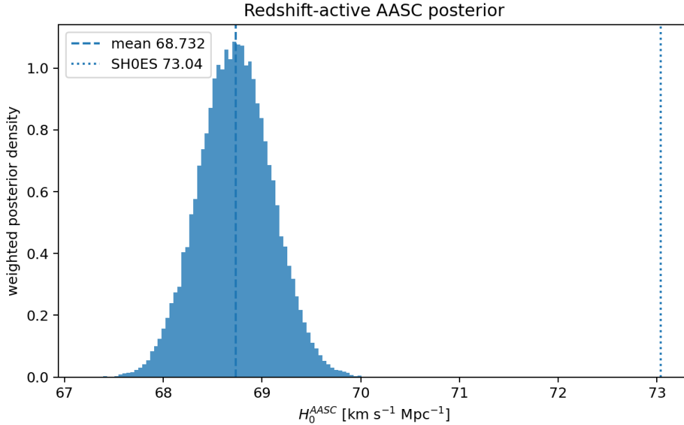
Figure 1: Primary redshift-active five-chain posterior for H_{0,RA}^{AASC} . The posterior remains in the Planck/BAO-supported region rather than migrating to the SH0ES central value.
