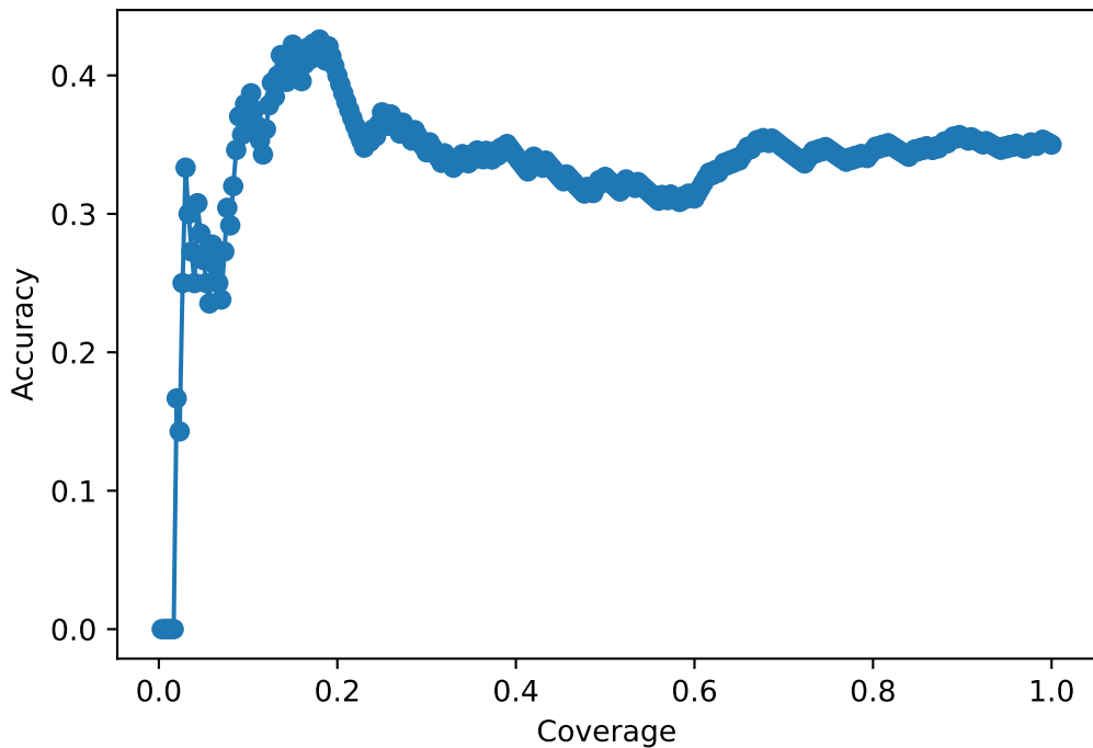
Risk-Coverage (Accuracy vs Coverage)
