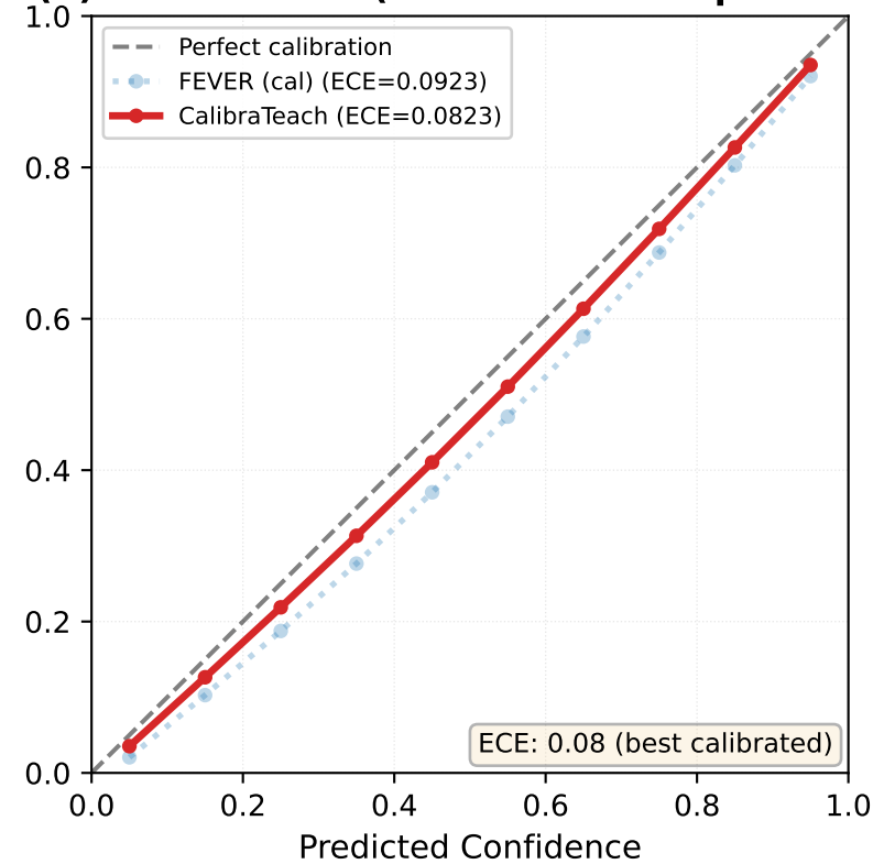
(C) CalibraTeach (Ensemble + Temperature)
