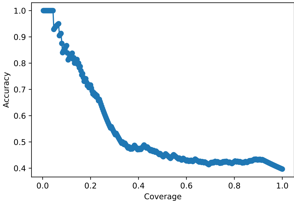
Risk-Coverage (Accuracy vs Coverage)
