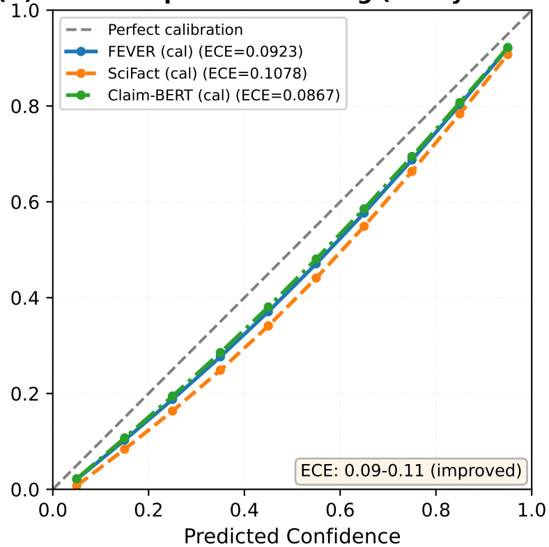
(B) After Temperature Scaling (Parity Protocol)
