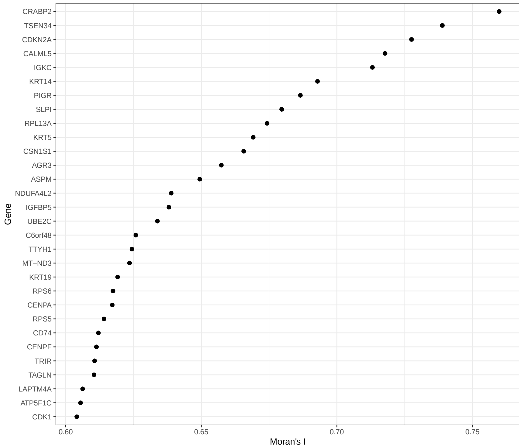
Top 30 Genes by Moran's I
