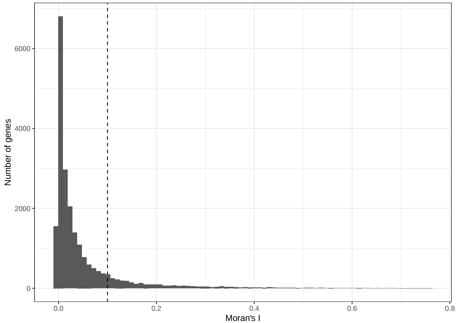
Distribution of Moran's I
