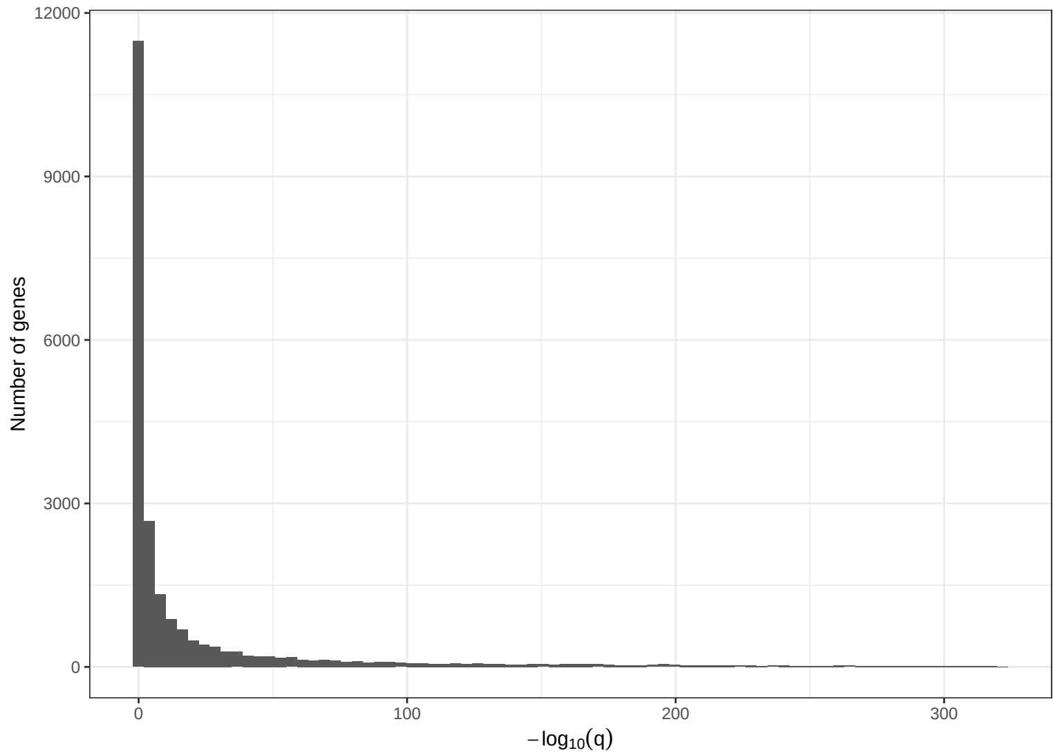
Distribution of graph_test q-values
