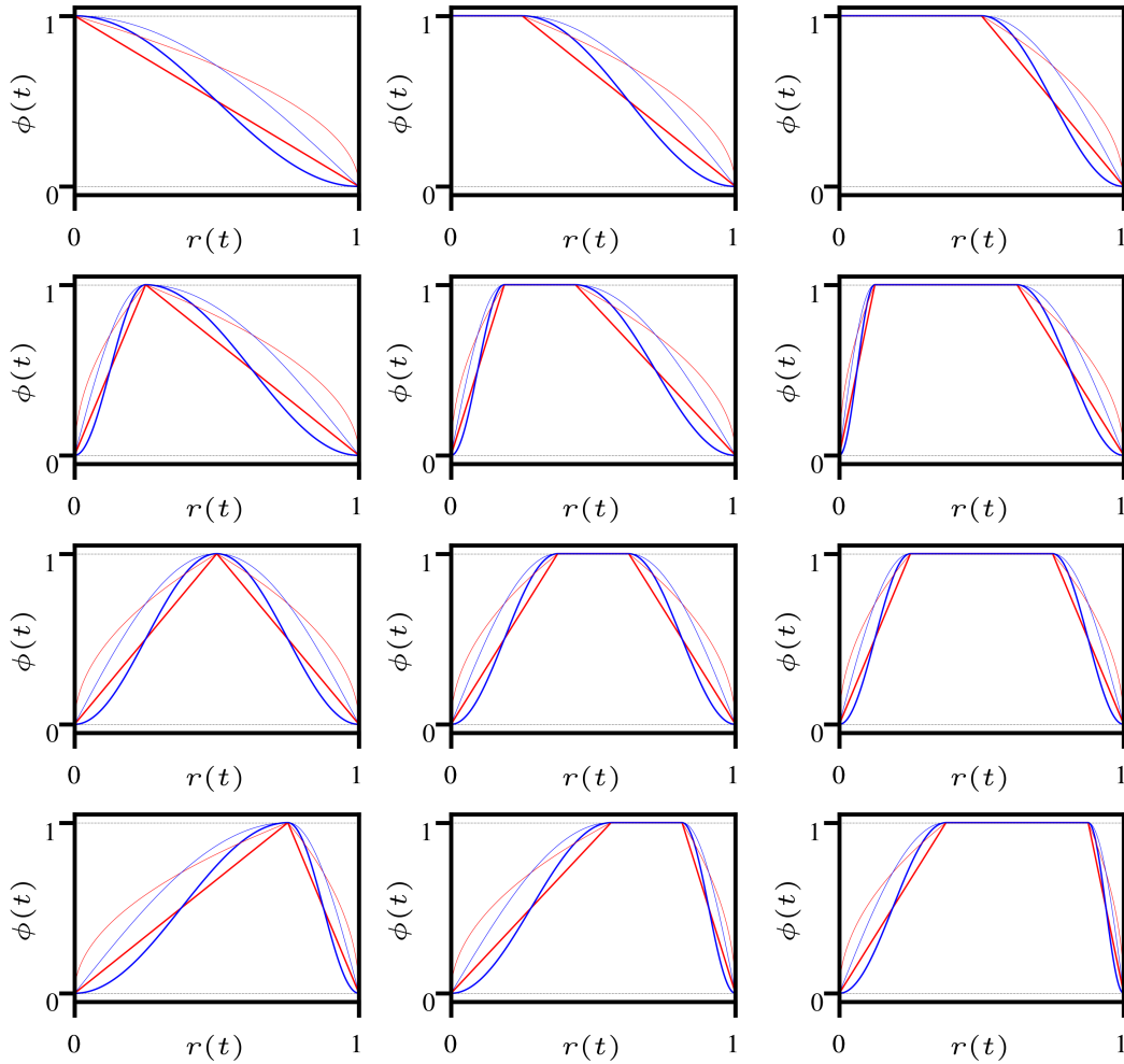
Figure 1: Window shapes obtained by passing x_4(r; m, \varepsilon) into the linear function 1 - x_4 (thick, red), raised-cosine function \cos^2(0.5 \pi x_4) (thick, blue) and their square-root forms (thin lines). Top row: m = 0 , \varepsilon = \{0, 0.25, 0.5\} (Left to Right). Second row: m = 0.25 , \varepsilon = \{0, 0.25, 0.5\} (Left to Right). Third row: m = 0.5 , \varepsilon = \{0, 0.25, 0.5\} (Left to Right). Bottom row: m = 0.75 , \varepsilon = \{0, 0.25, 0.5\} (Left to Right). Observe the variation from the default decay shapes (first row, first column) to the half-trapezoidal shapes (red, first row, second–third columns) to the triangular shapes (red, second–fourth rows, first column), and to the full-trapezoidal shapes (red, second–fourth rows, second–third columns).
