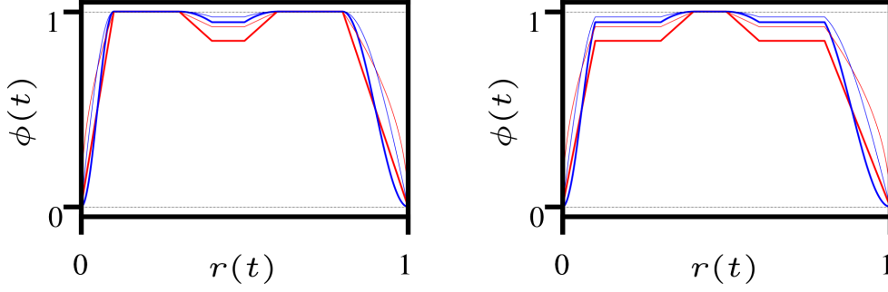
Figure 2: General M-shaped (left) and Dome-shaped (right) windows obtained from the 8-point boundary-value problem. Linear function 1 - x_8 (thick, red), raised-cosine function \cos^2(0.5 \pi x_8) (thick, blue) and their square-root forms (thin lines). Design parameters used for the shape generation are (m_1, \varepsilon_1, m_2, \varepsilon_2, m_3, \varepsilon_3, c) = (0.1, 0.2, 0.4, 0.1, 0.6, 0.2, 0.85) .
