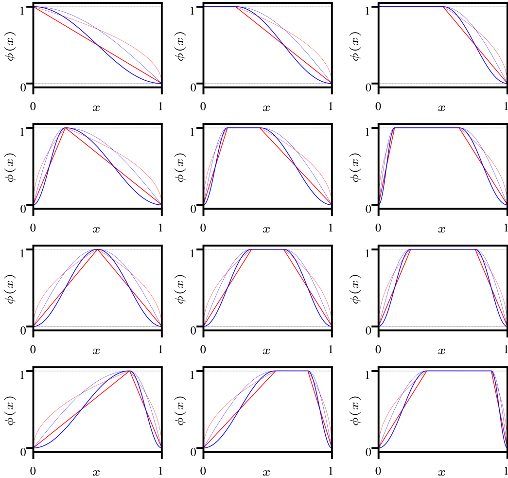
Figure 1: Window shapes obtained by passing x_4(r; m, \varepsilon) into the linear function 1 - x_4 (red), raised-cosine function \cos^2(0.5\pi x_4) (thick, blue) and their square-root forms (thin lines). Top row: m = 0 , \varepsilon = \{0, 0.25, 0.5\} (Left to Right). Second row: m = 0.25 , \varepsilon = \{0, 0.25, 0.5\} (Left to Right). Third row: m = 0.5 , \varepsilon = \{0, 0.25, 0.5\} (Left to Right). Bottom row: m = 0.75 , \varepsilon = \{0, 0.25, 0.5\} (Left to Right). Observe the variation from the default decay shapes (first row, first column) to the half-trapezoidal shapes (red, first row, second–third columns) to the triangular shapes (red, second–fourth rows, first column), and to the full-trapezoidal shapes (red, second–fourth rows, second–third columns).
