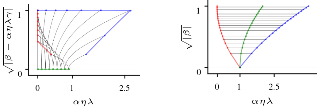
Figure 4: Left panel: Nesterov momentum ( \gamma = \beta/(1 + \beta) ): Equal eigenvalue magnitude |z_1| = |z_2| = \sqrt{|\beta - \alpha\eta\lambda\gamma|} < 1 of the stable expected error system versus the normalized learning rate \alpha\eta\lambda . Red and blue dots represent the minimum and maximum points of the stable learning rate intervals for any 0 \leq \beta < 1 . The green dots represent points where the equal-magnitude hits the origin |z_1| = |z_2| = 0 which indicate the fastest possible exponential decay rate to 0, and \alpha\eta\lambda = 1 + \beta . Plain SGM corresponds to the single dot ( \beta = 0, \alpha\eta\lambda = 1 ). Right panel: Heavy-ball momentum ( \gamma = 0 ): Equal eigenvalue magnitude |z_1| = |z_2| = \sqrt{|\beta|} < 1 versus the normalized learning rate \alpha\eta\lambda . This represents the fastest possible decay rate for the stable expected error system when \gamma = 0 . Red and blue dots represent the minimum and maximum points of the stable learning rate intervals for any 0 \leq \beta < 1 . The green dots represent the points where \alpha\eta\lambda = 1 + \beta . Plain SGM corresponds to the single dot ( \beta = 0, \alpha\eta\lambda = 1 ).
