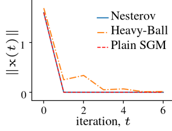
Figure 1: Ensemble average plot of the mean error dynamics \mathbf{x}(t) = \mathbf{A}^t \mathbf{x}(0) over 10000 independent trials. Evolution of the Euclidean norm \|\mathbf{x}(t)\|_2 of the two-state mean error dynamics in the one-dimensional stochastic error setup for the stochastic gradient learning algorithm is shown under three configurations: Plain form, Heavy-Ball momentum, and Nesterov momentum using the same random initialization \mathbf{x}(0) , \lambda = 1 , and \kappa = 1 . For momentum, \beta = 0.2 was used. Fastest mean convergence is achieved both with or without momentum.
