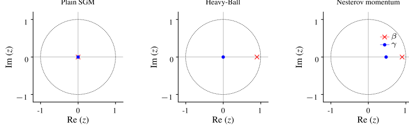
Figure 3: Illustrative Pole-zero locations in the complex z -plane for plain stochastic gradient descent (SGM), Heavy-Ball momentum (HB), and Nesterov momentum (NAG). HB introduces a single stable pole with a zero at the origin, while NAG places a zero inside the unit circle relative to the same pole.
