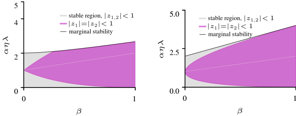
Figure 4: Stability regions in the (\beta, \alpha\eta\lambda) plane for Nesterov momentum (left) and Heavy-Ball momentum (right) given 0 \leq \beta < 1 . Gray shading marks the Jury-stability region where both eigenvalues satisfy |z_{1,2}| < 1 , the magenta area marks the stricter equal-magnitude region |z_1| = |z_2| < 1 , and the black curve shows the marginal stability boundary |z_1| = |z_2| = 1 . For Nesterov momentum , the dotted thin white lines inside the magenta-colored area marks the closed-form parameterization for the fastest possible exponential decay rate |z_1| = |z_2| = \sqrt{|\beta - \alpha\eta\lambda\gamma|} = 0 of the mean error dynamics. For the Heavy-Ball momentum parameterization, the magenta area marks a stricter equal-magnitude region |z_1| = |z_2| = \sqrt{|\beta|} < 1 corresponding to its fastest possible exponential decay of the mean-error dynamics, the thin white lines mark the points where \alpha\eta\lambda = 1 + \beta . The (\beta, \alpha\eta\lambda) plane shows how both design choices expands and reshapes the range of stable learning-rates compared to the single dot ( \beta = 0 ) of the plain SGM, reflecting the lowpass regularization effect of momentum.
