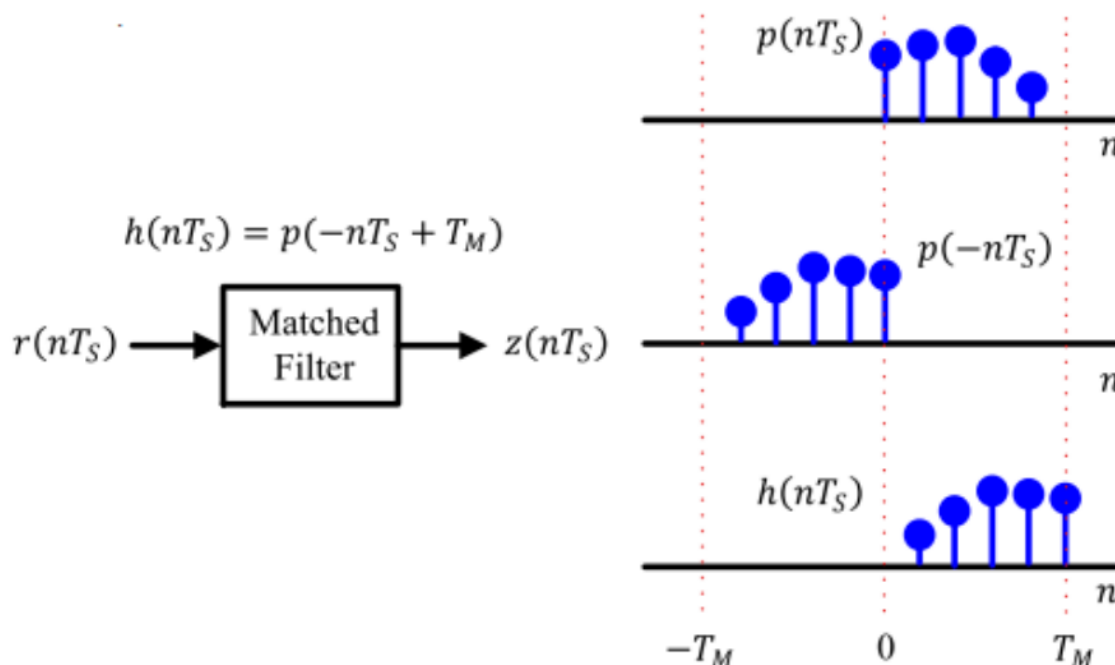
Рис. 28 — Matched filter
