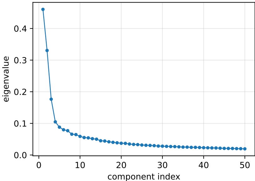
RBF Kernel PCA scree ( \gamma=1/d , n=5000 )
