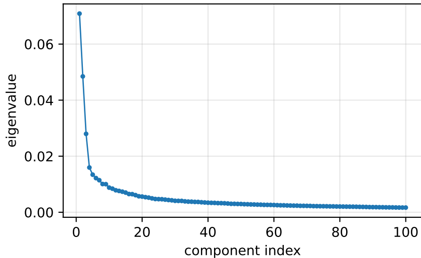
Scree plot (top 100)
