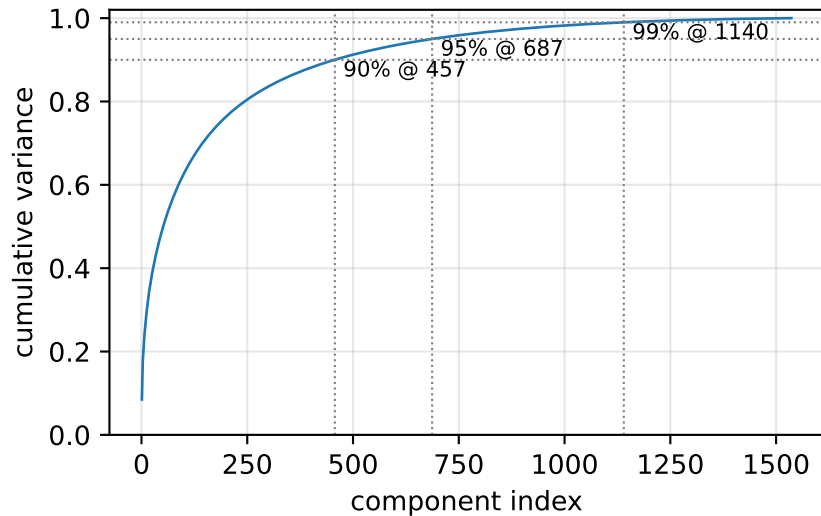
Cumulative variance
